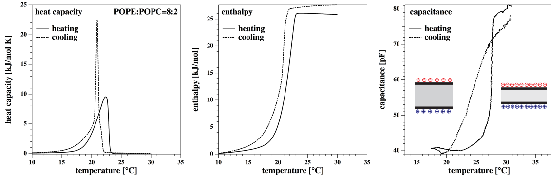
Figure 2. Left: Melting profile of a POPE : POPC = 8:2 membrane. Shown are both heating and cooling scans. Scan rate was 5°/hour. Center: The integral of the heat capacities yields the enthalpy changes. Right: In BLM experiments, one finds significant changes of the membrane capacitance of 89%.
