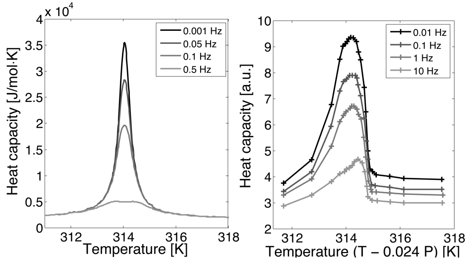
Figure 5: Left : The calculated dynamic heat capacity for LUV of DPPC at different frequencies. Right : The effective heat capacity profiles for LUV of DPPC at different frequencies, measured by Van Osdol et al. [19]. The measured effective heat capacities have not been corrected for contributions from the experimental setup, and a direct comparison is therefore not possible. The theoretical dynamic heat capacity shows the same qualitative features as the measurements — a dramatic decrease in the height of the excess heat capacity with increasing frequency and a relatively constant width. The difference in frequency scales seen in the two panels is due to an estimated difference of more than a factor of 10 in the characteristic relaxation time. Frequencies are given in units of \text{Hz} = (1/2\pi) \text{ rad/s} .
