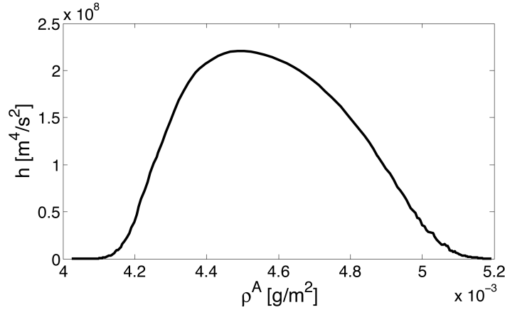
Figure 4: The dispersion parameter, h , as a function of lateral density for LUV of DPPC, based on the proposed expression for the lateral speed of sound.
