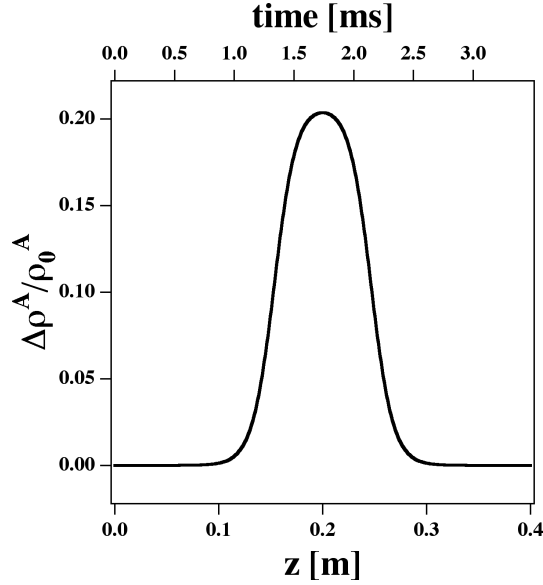
Figure 1: The propagating soliton using parameters appropriate for unilamellar DPPC vesicles and a dispersion constant h = 2 \text{ m}^4/\text{s}^2 (from [21]). The soliton has a width of about 10 cm and a duration of about 1 ms, which is very similar to action potentials in myelinated nerves.
