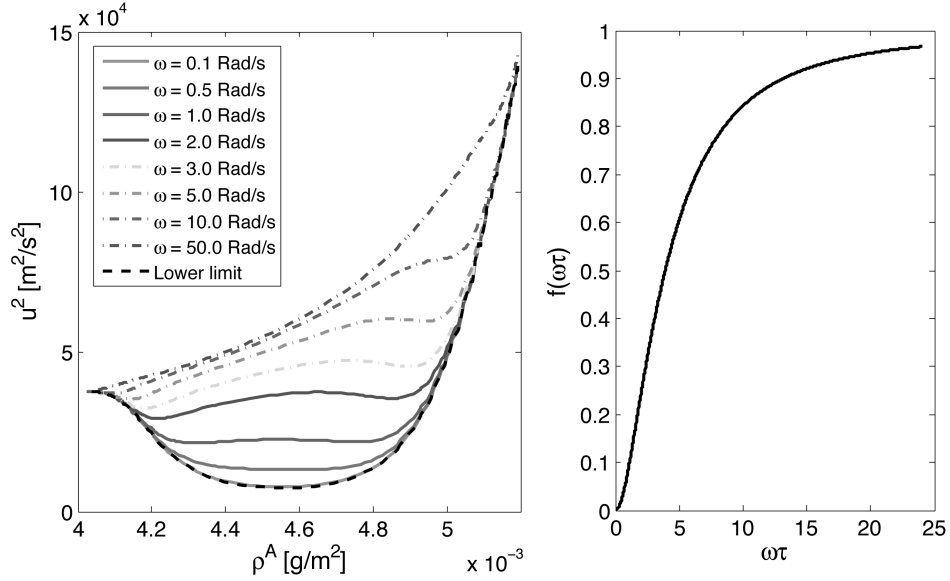
Figure 3: Left : The effective lateral speed of sound squared as a function of density at different angular frequencies along with the limiting case: \omega \rightarrow 0 . Right : The generic function, f(\omega\tau) , that takes the effective lateral speed of sound squared, at a given lateral density, from the low frequency limit ( f(\omega\tau \rightarrow 0) = 0 ) to the high frequency limit ( f(\omega\tau \rightarrow \infty) = 1 ).
