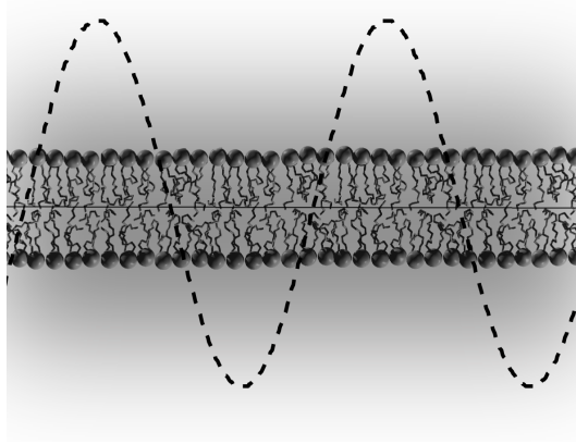
Figure 2: Visualization of temperature wave in the plane of a lipid bilayer. The coloring indicates heat penetrating into the surrounding water.
