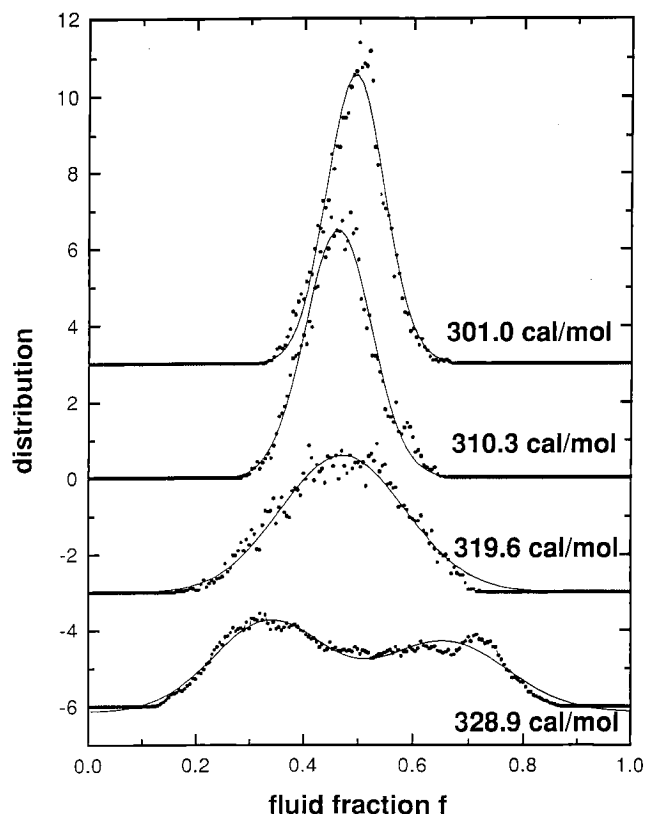
FIGURE 3 Distribution of states during a Monte Carlo simulation at the heat capacity maximum, from top to bottom with \Delta\omega_{gl} = 301.0, 310.3, 319.6 , and 328.9 cal/mol. All other parameters as in Fig. 2. The bottom curve has more than one maximum, indicative of a first-order transition. All other curves represent second order transitions (see text). Solid curves are fits with one-component or two-component (bottom) Gaussian distributions.
