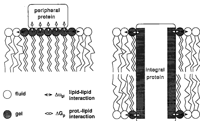
FIGURE 1 Schematic picture of lipid-protein association. Local interactions \Delta\omega_{gl} and \Delta G_p for peripheral (left) and integral proteins (right) are indicated with solid and open arrows, respectively.
