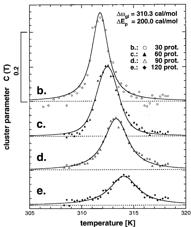
FIGURE 6 Protein cluster parameter defined through Eq. 8, demonstrating the effect of domain formation on the protein distribution at the lipid/protein ratios and thermodynamic parameters as in Fig. 4 a . Symbols are the same as in Fig. 4 a . The aggregation exhibits a pronounced maximum close to the heat capacity maximum.
