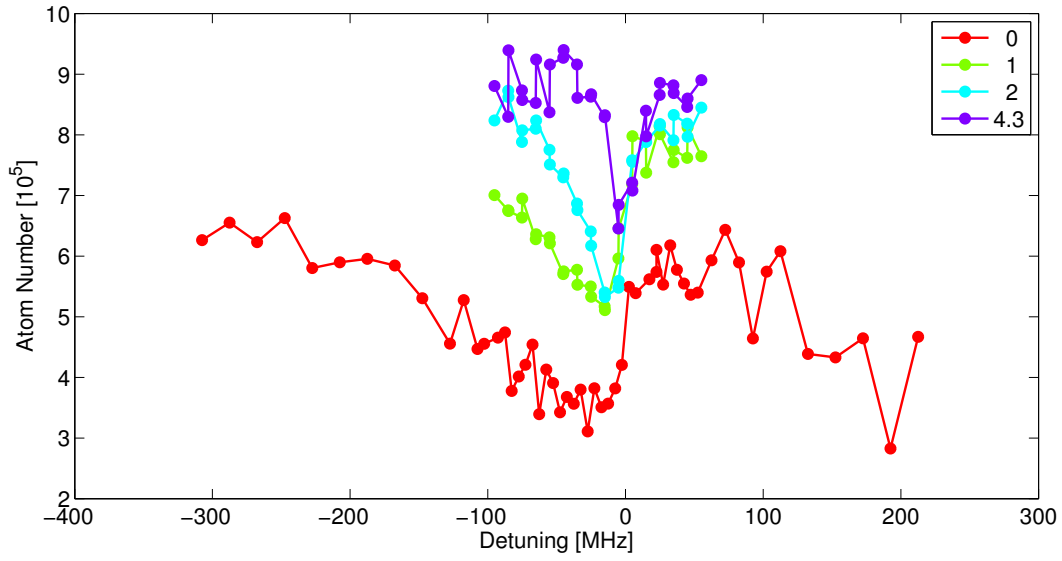
Figure 13.2: Atom loss spectrum of a BEC as determined from absorption images after 45ms TOF. The loss is induced by a probe beam, which is applied after various TOF with an intensity of I = 0.42 \text{ W/m}^2 . The BEC has an in-trap density of \rho = 1.4 \cdot 10^{20} \text{ m}^{-3} . The atom number without probe in the BEC is N_{at} = 6.1 \cdot 10^5 , the total atom number is N_{at} = 9.6 \cdot 10^5 . The data set with 0ms TOF has slightly different parameters, The density is \rho = 1.3 \cdot 10^{20} \text{ m}^{-3} , the BEC atom number is N_{at} = 4.9 \cdot 10^5 and the total atom number is N_{at} = 7.4 \cdot 10^5 .
