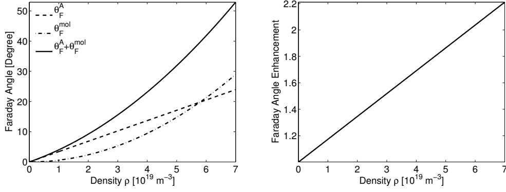
Figure 6.7: Left: Faraday angle as a function of density at a detuning of \Delta_A = -600 \text{ MHz} . The atomic Faraday angle \theta_F^A increases linearly while the molecular \theta_F^{\text{mol}} scales as density squared. Right: Resulting Faraday angle enhancement factor (\theta_F^A + \theta_F^{\text{mol}})/\theta_F^A due to interactions between two atoms at the -600MHz detuning.
