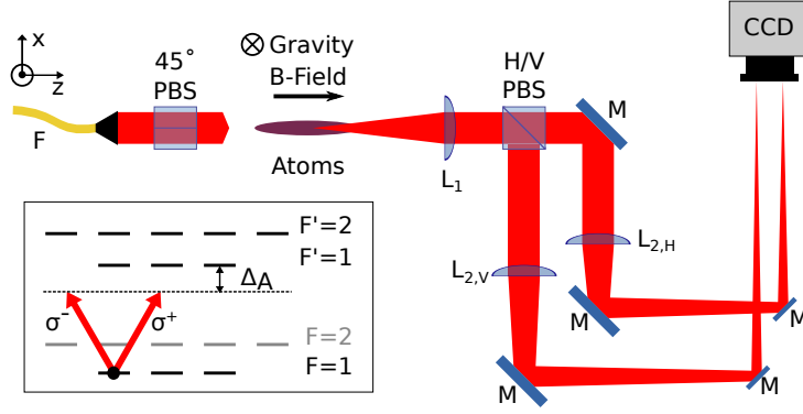
Figure 11.1: Optical setup showing the 45^\circ PBS preparing the probe light after the Fiber (F), the placement of lenses L_1 , L_{2,H} and L_{2,V} , mirrors (M) and analyzing cube H/V PBS as well as the CCD camera. The B-field direction is mainly along z . The inset shows the ^{87}\text{Rb} D1 line level scheme and the linear probe light in the z quantization axis.
