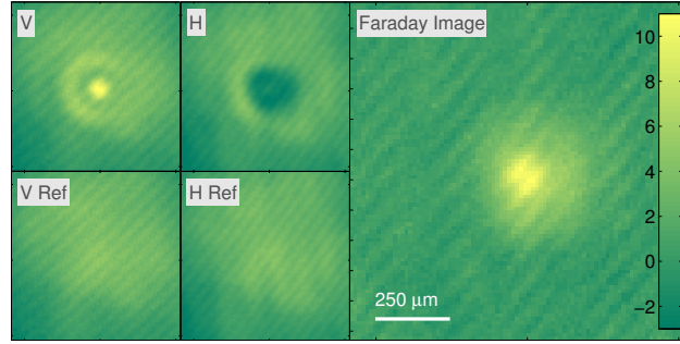
Figure 11.5: Raw images (left panel) and deduced Faraday image (right panel) for a detuning of \Delta_A / (2\pi) = -400\text{MHz} . V/H refers to images with atoms present, while V/H Ref to images without atoms. The color scale indicates the Faraday angle in degrees. Diffraction rings in the raw images V/H disappear in the Faraday image.
