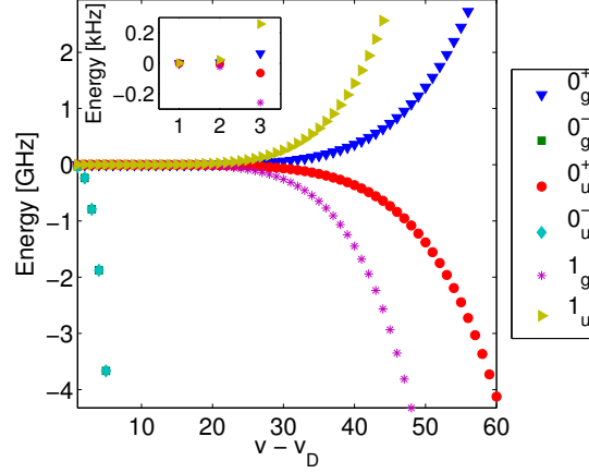
Figure C.2: LeRoy-Bernstein energies of the D1 line potentials relevant for our experiments. The inset shows the energies close to the dissociation limit.
