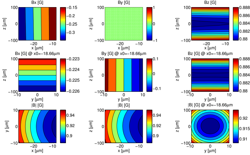
Figure B.2: Ioffe-Pritchard magnetic field configuration at the sagged position of the atomic ensemble x_{\text{sag}} = -18.66 \mu\text{m} . The top row figure in the middle column
