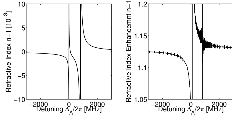
Figure 6.8: Refractive index deviation ( n-1 ) due to non-interacting atoms (left) and the enhancement of ( n-1 ) due to interactions. The peak density is \rho_0 = 2.64 \times 10^{19} \text{ m}^{-3}
