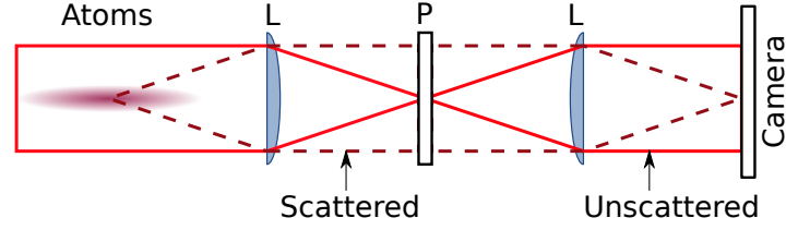
Figure 5.6: General setup used for dispersive imaging. The unscattered light will be focused onto the Fourier plane between the two lenses (L) while the scattered light is not. An optical element P is used in the Fourier plane to modify the unscattered light. A camera captures the image. P can be a phase-plate, a polarizer, a light block or a polarizing beam-splitter.
