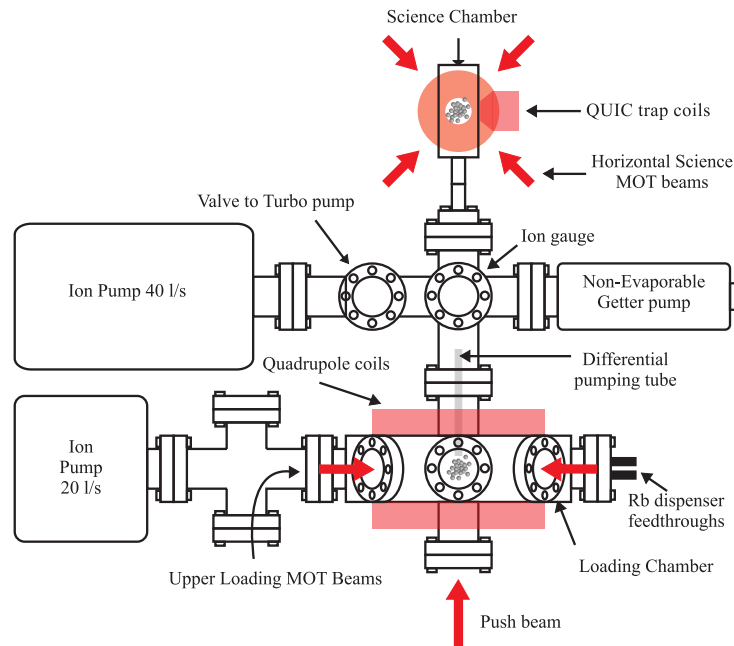
Figure 8.1: Top view of the two chamber vacuum system with ion pumps, dispensers, the differential pumping stage, and the coils for MOTs and magnetic trap. Indicated are also the laser beams for the MOT operation.
